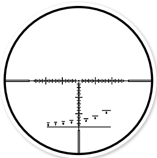
DMR8i RETICLE SUBTENSIONS
